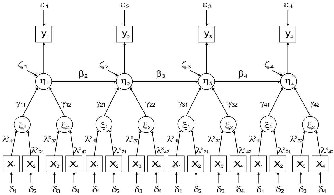
Figure 6 – The GENERAL SIMPLEX model path diagram.
